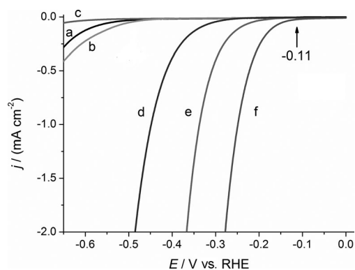
Figure 3. Polarization curves of a) bare GCE, b) bare GCE coated with Nafion, c) C_{60} modified GCE, d) C_{60}(OH)_8 modified GCE, e) C_{60}(OH)_8 anion salt modified GCE, and f) Nafion/ C_{60}(OH)_8 salt/GCE. All performed in H_2SO_4 (0.5 M) at a scan rate of 2 mV s^{-1} . See the Supporting Information for experimental details.
